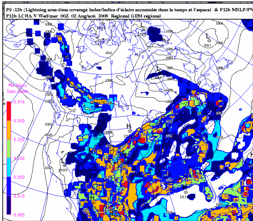
Figure 11. 9-12 hour forecast of the time-area coverage index (LCHA) valid for 2100 UTC 01 August 2006 to 0000 UTC 02 August 2006.
