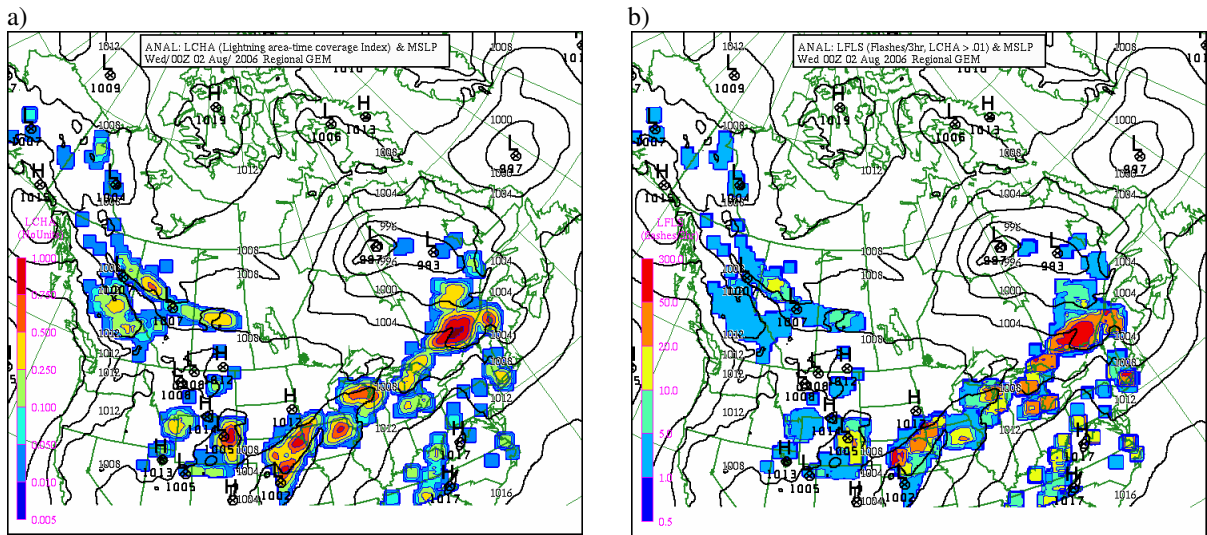
Figure 10. Observed a) time-area coverage index (LCHA); b) three-hour flash count (LFLS) for 2100 – 2400 UTC 01 August 2006. MSLP pressure is overlain. Only the lightning reports received by Environment Canada are shown.
