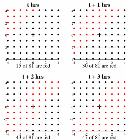
Figure 2. The 9*9 point smoothing grid surrounding grid point ( i,j ), indicated with “+”, and applied at forecast times t, t_{+1hr}, t_{+2hr}, t_{+3hr} .
