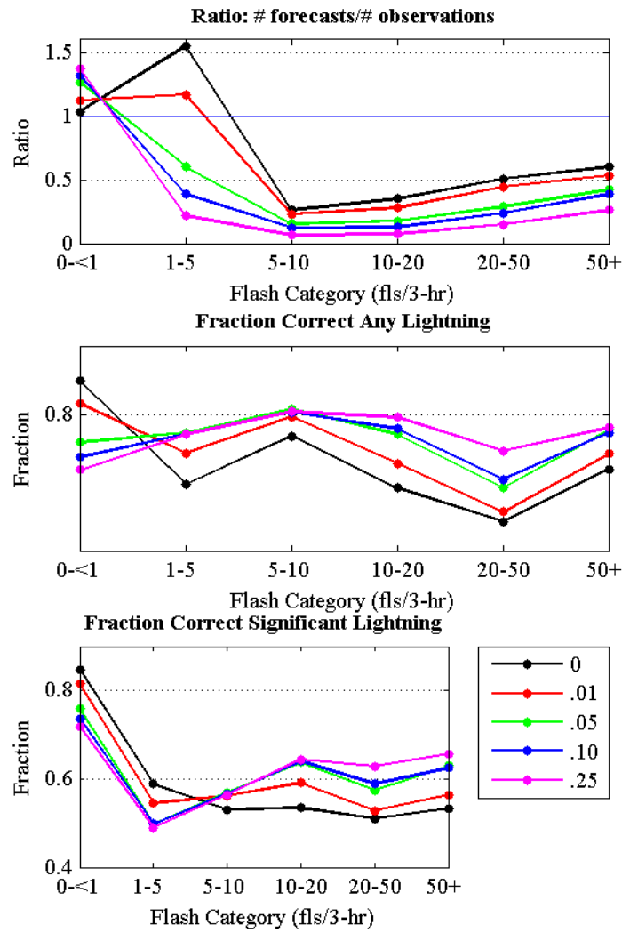
Figure 18. The ratio of forecasts to observations and the fraction correct for any lightning and significant lightning for 12-hr forecasts valid 2100-2400 UTC July 2006, where the verifying observations of LCHA and LFLS are the maximum value in the 324 data point cloud.
