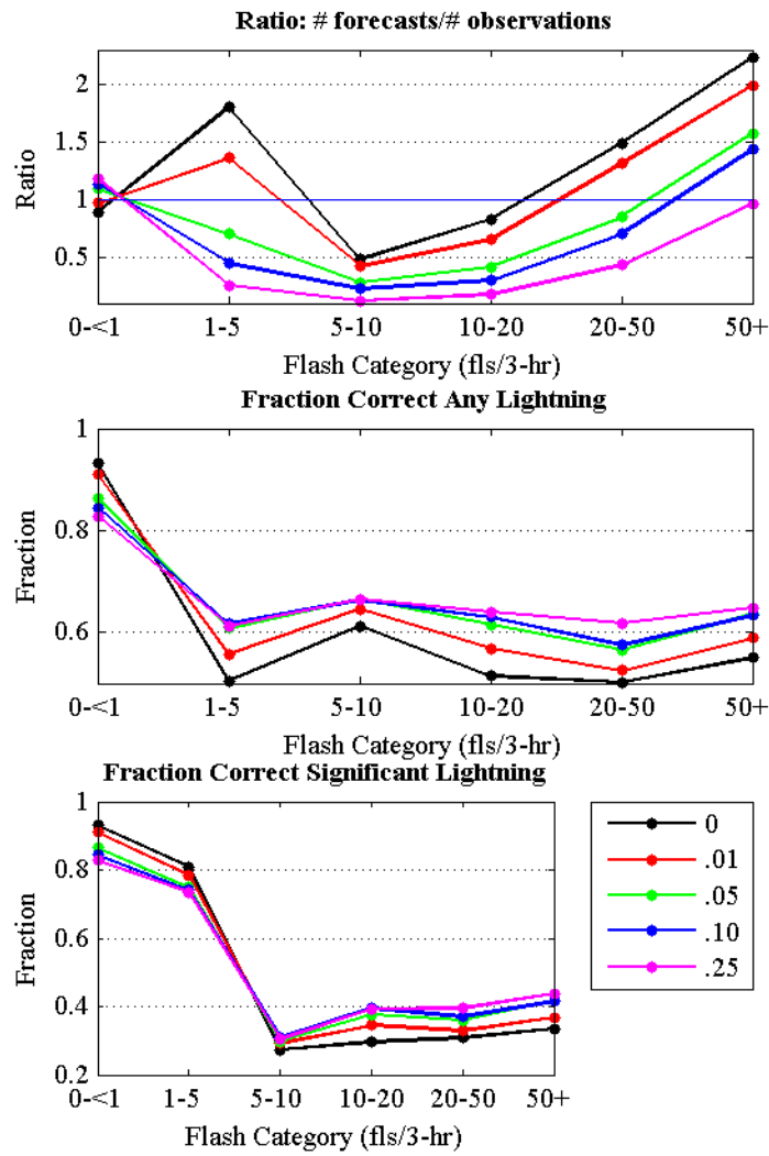
Figure 17. The ratio of forecasts to observations and the fraction correct for any lightning and significant lightning for 12-hr forecasts valid 2100-2400 UTC July 2006.
